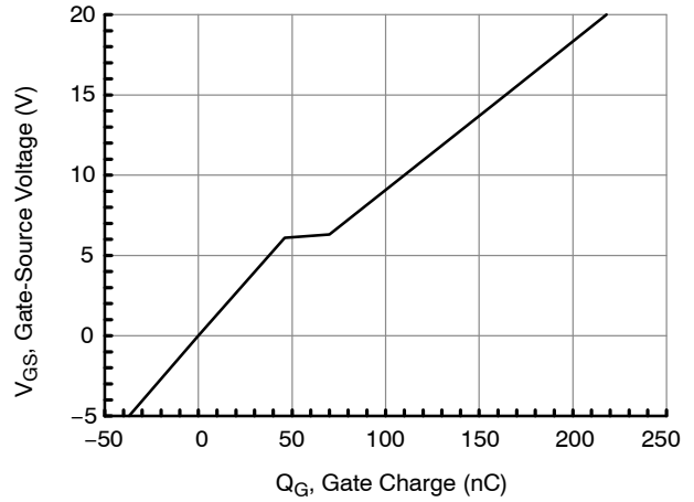
Figure 8. Typical Gate Charge at V_{DS} = 400\text{ V} and I_D = 80\text{ A}
