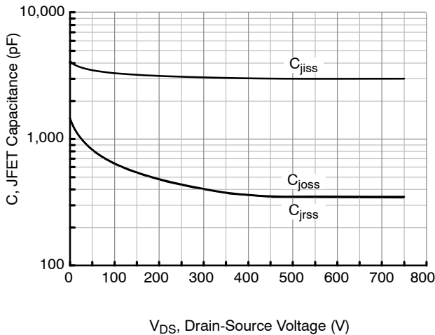
Figure 23. Typical JFET Capacitances at f = 100\text{ kHz} and V_{JGS} = -20\text{ V}
