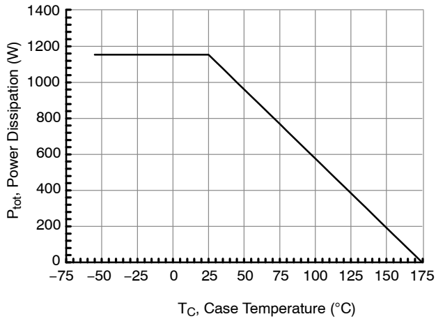
Figure 15. Total Power Dissipation
