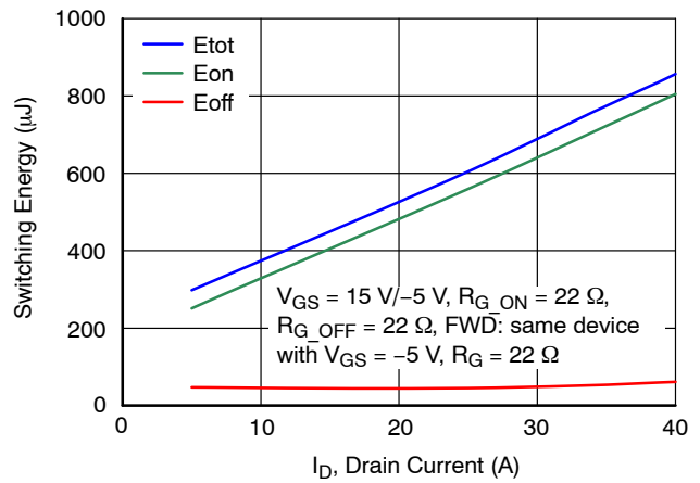
Figure 18. Clamped Inductive Switching Energy vs. Drain Current at V_{DS} = 800 \text{ V} and T_J = 25 \text{ }^\circ\text{C}
