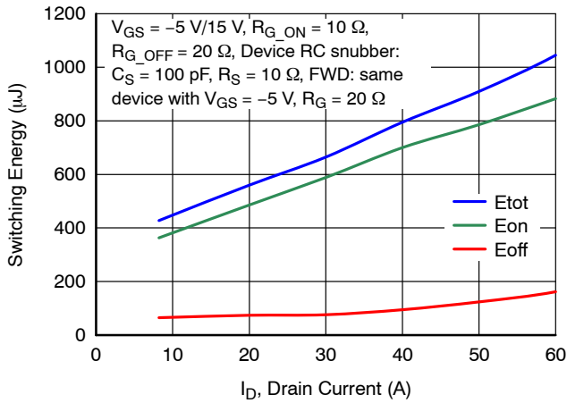
Figure 19. Clamped Inductive Switching Energy vs. Drain Current at V_{DS} = 800\text{ V} and T_J = 25\text{ °C}
