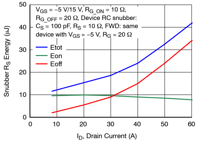
Figure 20. RC Snubber Energy Loss vs. Drain Current at V_{DS} = 800\text{ V} and T_J = 25\text{ °C}
