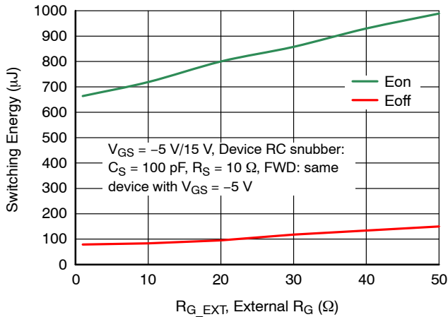
Figure 21. Clamped Inductive Switching Energies vs. R_{G,EXT} at V_{DS} = 800\text{ V} , I_D = 40\text{ A} , and T_J = 25\text{ °C}
