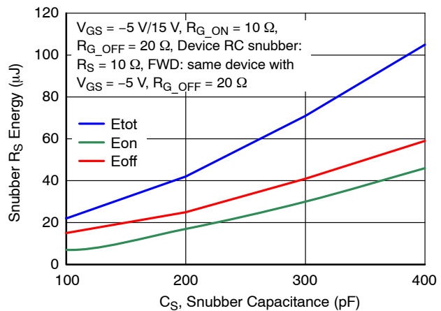
Figure 24. RC Snubber Energy Losses vs. Snubber Capacitance C_S at V_{DS} = 800\text{ V} , I_D = 40\text{ A} , and T_J = 25\text{ °C}
