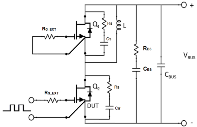
Figure 26. Schematic of the Half-bridge Mode Switching Test Circuit with Device RC Snubbers ( R_S = 10\ \Omega , C_S = 100\text{ pF} ) and a Bus RC Snubber ( R_{BS} = 2.5\ \Omega , C_{BS} = 100\text{ nF} )
