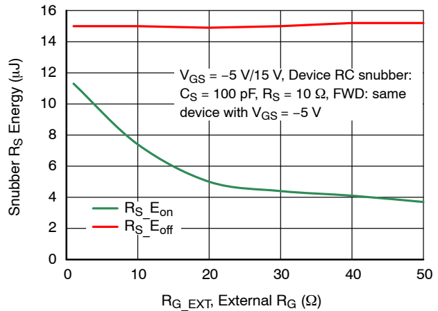
Figure 22. RC Snubber Energy Loss vs. R_{G,EXT} at V_{DS} = 800\text{ V} , I_D = 40\text{ A} , and T_J = 25\text{ °C}
