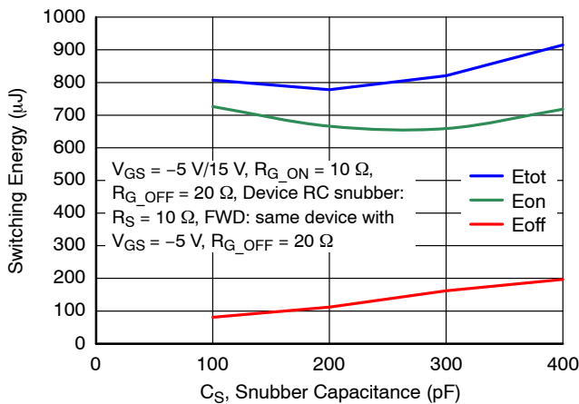
Figure 23. Clamped Inductive Switching Energies vs. Snubber Capacitance C_S at V_{DS} = 800\text{ V} , I_D = 40\text{ A} , and T_J = 25\text{ °C}
