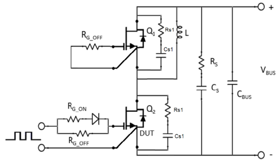
Figure 23. Schematic of the Half-Bridge Mode Switching Test Circuit with Device RC Snubbers ( R_{S1} = 10\text{ }\Omega , C_{S1} = 95\text{ pF} ) and a Bus RC Snubber ( R_S = 2.5\text{ }\Omega , C_S = 100\text{ nF} )
