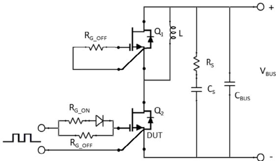
Figure 22. Schematic of the Half-Bridge Mode Switching Test Circuit. Note, a Bus RC Snubber ( R_S = 2.5\text{ }\Omega , C_{BS} = 100\text{ nF} ) is Used to Reduce the Power Loop High Frequency Oscillations
