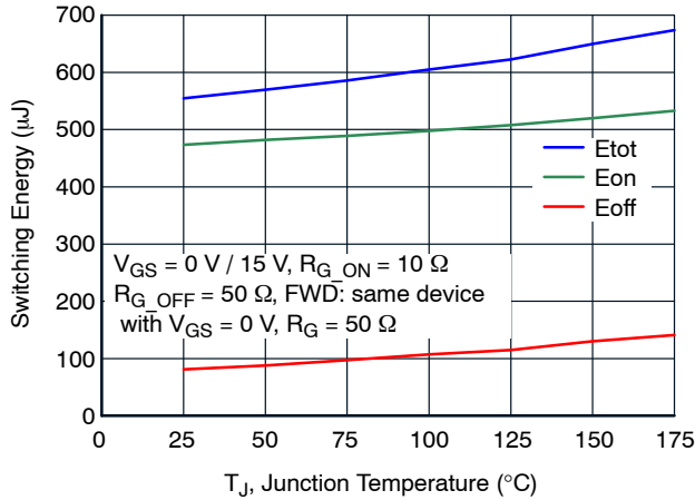
Figure 21. Clamped Inductive Switching Energies vs. Junction Temperature at V_{DS} = 800\text{ V} and I_D = 20\text{ A}
