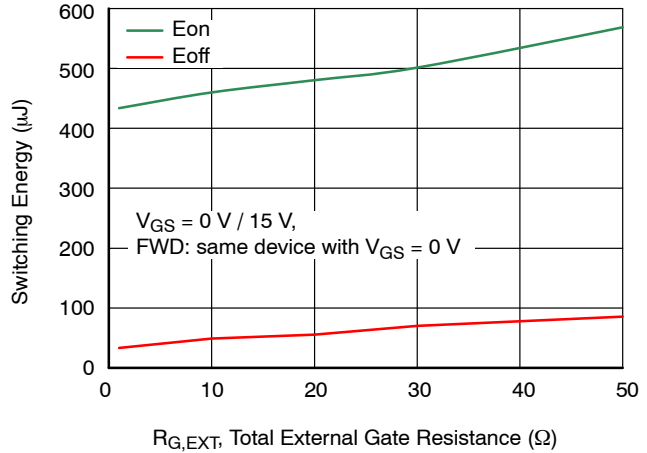
Figure 20. Clamped Inductive Switching Energies vs. R_{G,EXT} at V_{DS} = 800\text{ V} , I_D = 20\text{ A} , and T_J = 25\text{ }^\circ\text{C}
