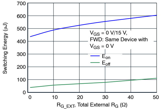
Figure 20. Clamped Inductive Switching vs. R_{G\_EXT} at V_{DS} = 800\text{ V} , I_D = 20\text{ A} and T_J = 25\text{ °C}
