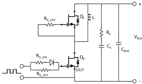
Figure 22. Schematic of the Half-Bridge Mode Switching Test Circuit. Note, a Bus RC Snubber ( R_S = 2.5 \Omega , C_S = 100 \text{ nF} ) Is Used To Reduce the Power Loop High Frequency Oscillations
