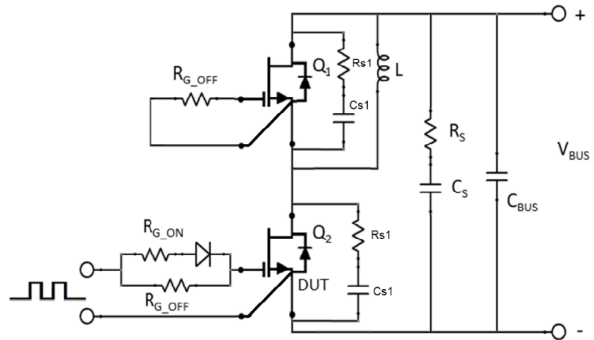
Figure 23. Schematic of the Half-Bridge Mode Switching Test Circuit with Device RC Snubber ( R_{S1} = 5\text{ } \Omega , C_{S1} = 95\text{ pF} ) and a Bus RC Snubber ( R_S = 2.5\text{ } \Omega , C_S = 100\text{ nF} )
