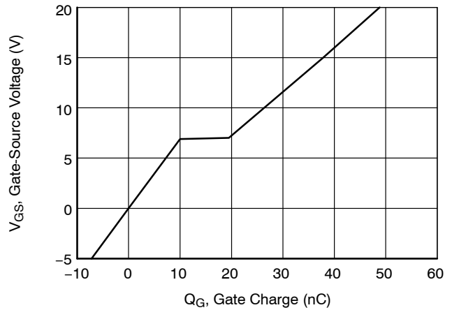
Figure 8. Typical Gate Charge at V_{DS} = 800\text{ V} and I_D = 25\text{ A}
