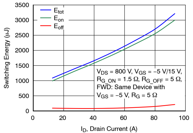
Figure 18. Clamped Inductive Switching Energy vs. Drain Current at T_J = 25 ^{\circ}C
