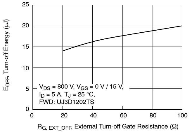
Figure 22. Clamped Inductive Switching Turn-off Energy vs. R_{G, EXT\_OFF}
