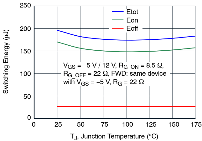
Figure 21. Clamped Inductive Switching Energy vs. Junction Temperature at V_{DS} = 800\text{ V} , and I_D = 13\text{ A}
