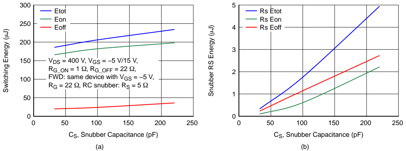
Figure 23. Clamped Inductive Switching Energy Including RC Snubber Energy Loss (a) and RC Snubber Energy Loss (b) as a Function of Snubber Capacitance at I_D = 20\text{ A} and T_J = 25\text{ }^\circ\text{C}
