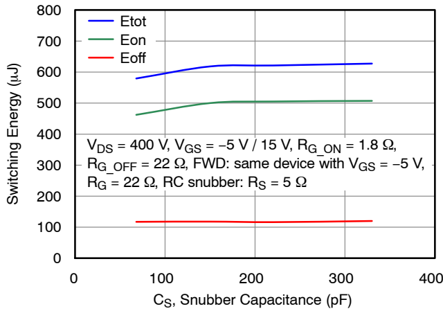
Figure 27. Clamped Inductive Switching Energy including RC Snubber Energy Loss as a Function of Snubber Capacitance at I_D = 40\text{ A} and T_J = 25\text{ }^\circ\text{C}
