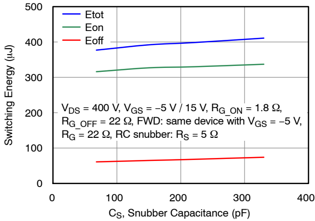
Figure 27. Clamped Inductive Switching Energy including RC Snubber Energy Loss as a Function of Snubber Capacitance at I_D = 30\text{ A} and T_J = 25\text{ }^\circ\text{C}
