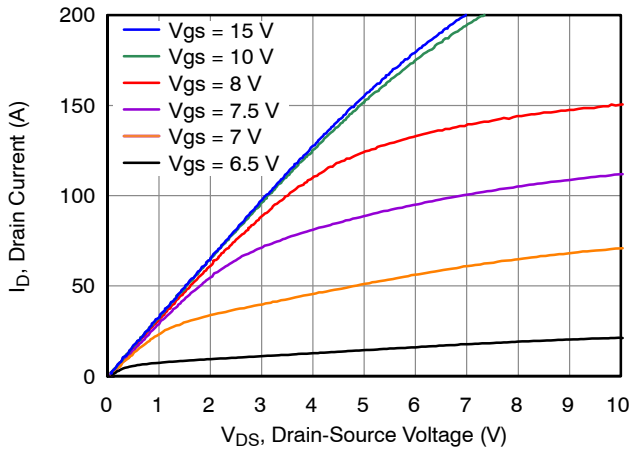
Figure 1. Typical Output Characteristics at T_J = -55\text{ }^\circ\text{C} , t_p < 250\ \mu\text{s}
