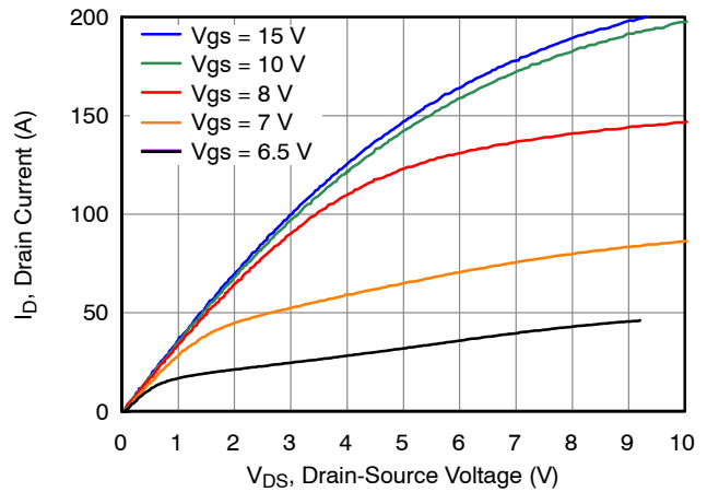
Figure 2. Typical Output Characteristics at T_J = 25\text{ }^\circ\text{C} , t_p < 250\ \mu\text{s}
