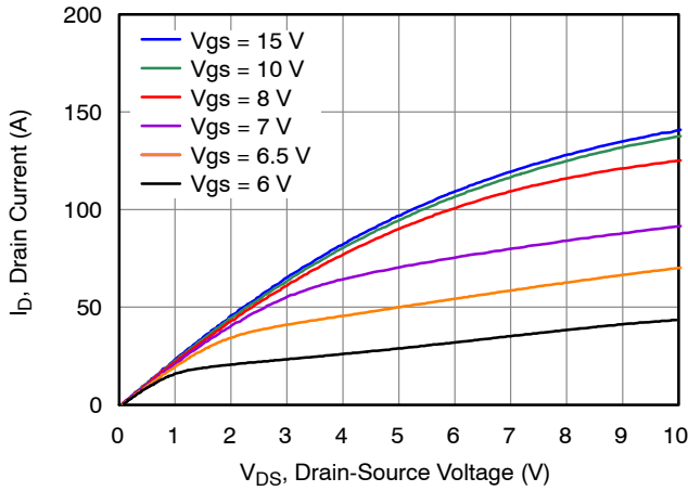
Figure 3. Typical Output Characteristics at T_J = 175\text{ }^\circ\text{C} , t_p < 250\ \mu\text{s}
