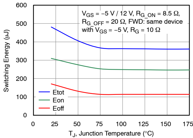
Figure 21. Clamped Inductive Switching Energy vs. Junction Temperature at V_{DS} = 400 V and I_D = 50 A
