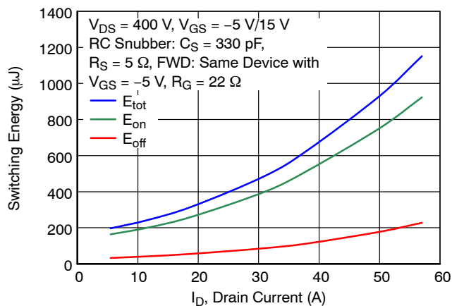
Figure 19. Clamped Inductive Switching Energy vs. Drain Current at T_J = 25 °C, Turn-on R_{G\_EXT} = 1.8 \Omega , and Turn-off R_{G\_EXT} = 22 \Omega
