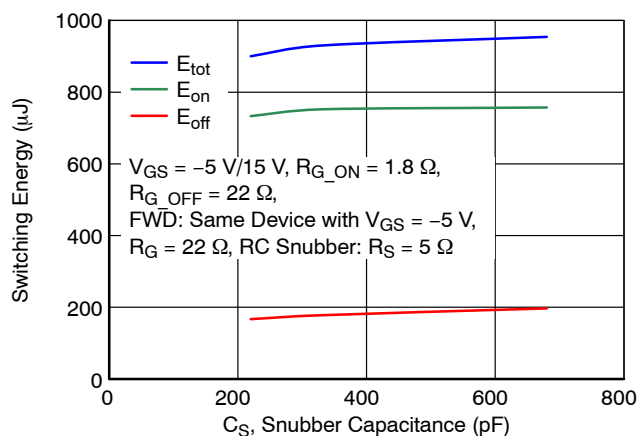
Figure 27. Clamped Inductive Switching Energy Including RC Snubber Energy Loss as a Function of Snubber Capacitance at I_{\text{D}} = 50 \text{ A} , V_{\text{DS}} = 400 \text{ V} , and T_J = 25 \text{ }^{\circ}\text{C}
