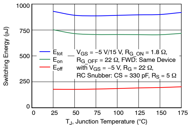
Figure 25. Clamped Inductive Switching Energy Including RC Snubber Energy Loss as a Function of Junction Temperature at I_{\text{D}} = 50 \text{ A} and V_{\text{DS}} = 400 \text{ V}
