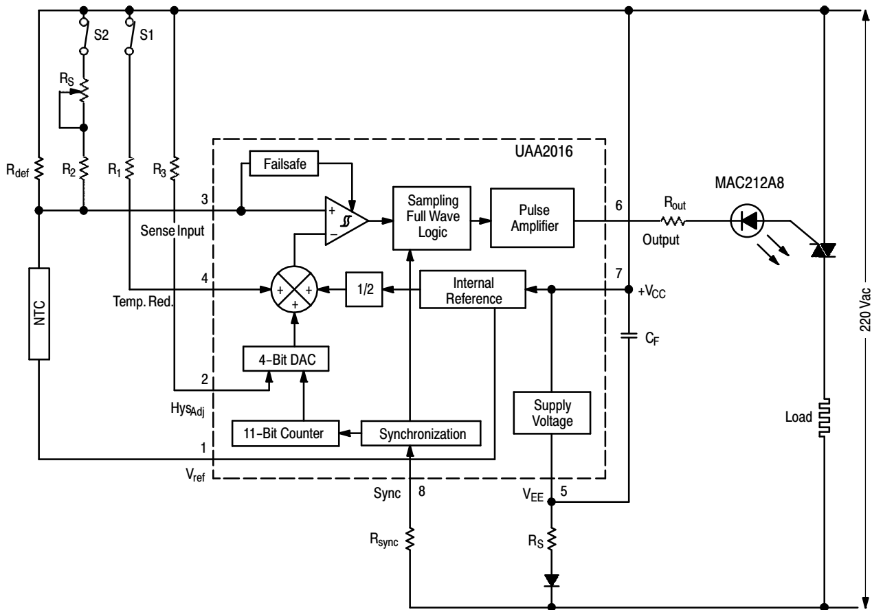
Figure 1. Application Schematic
