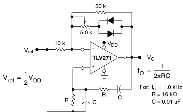
Figure 41. Wien Bridge Oscillator
