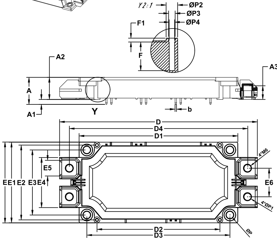
PIM11, 152.00x62.15x17.00 CASE 180HT ISSUE E
