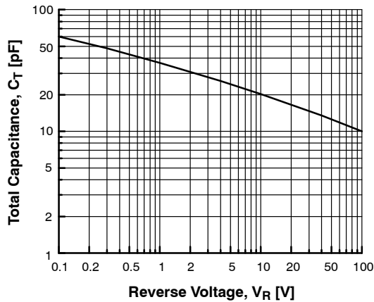
Figure 5. Total Capacitance
