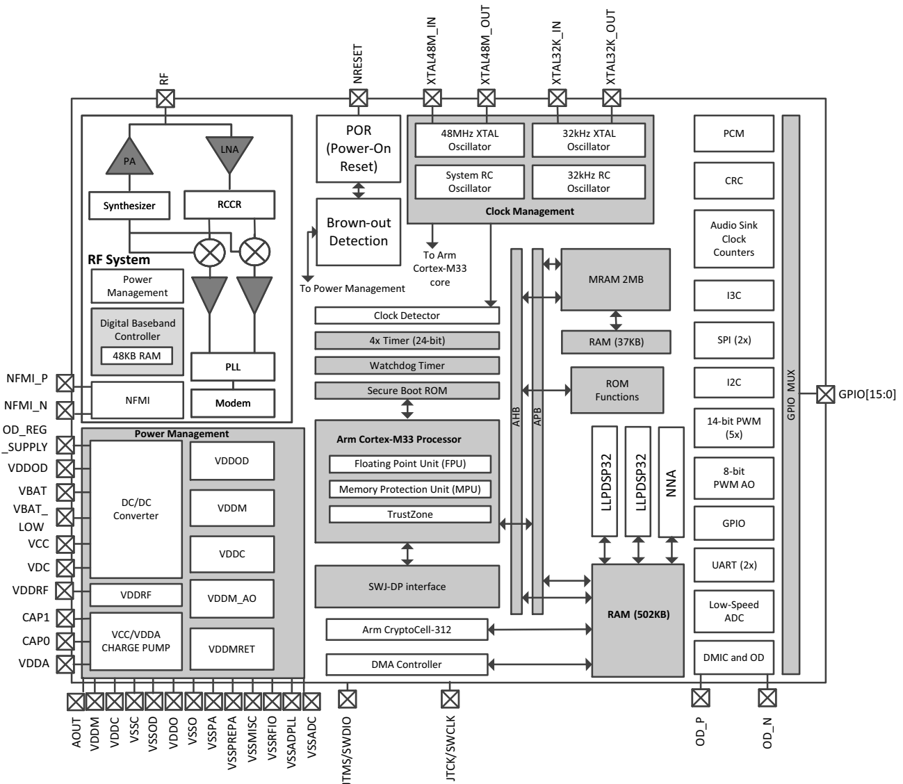
Figure 1. RSL20 Detailed Block Diagram
