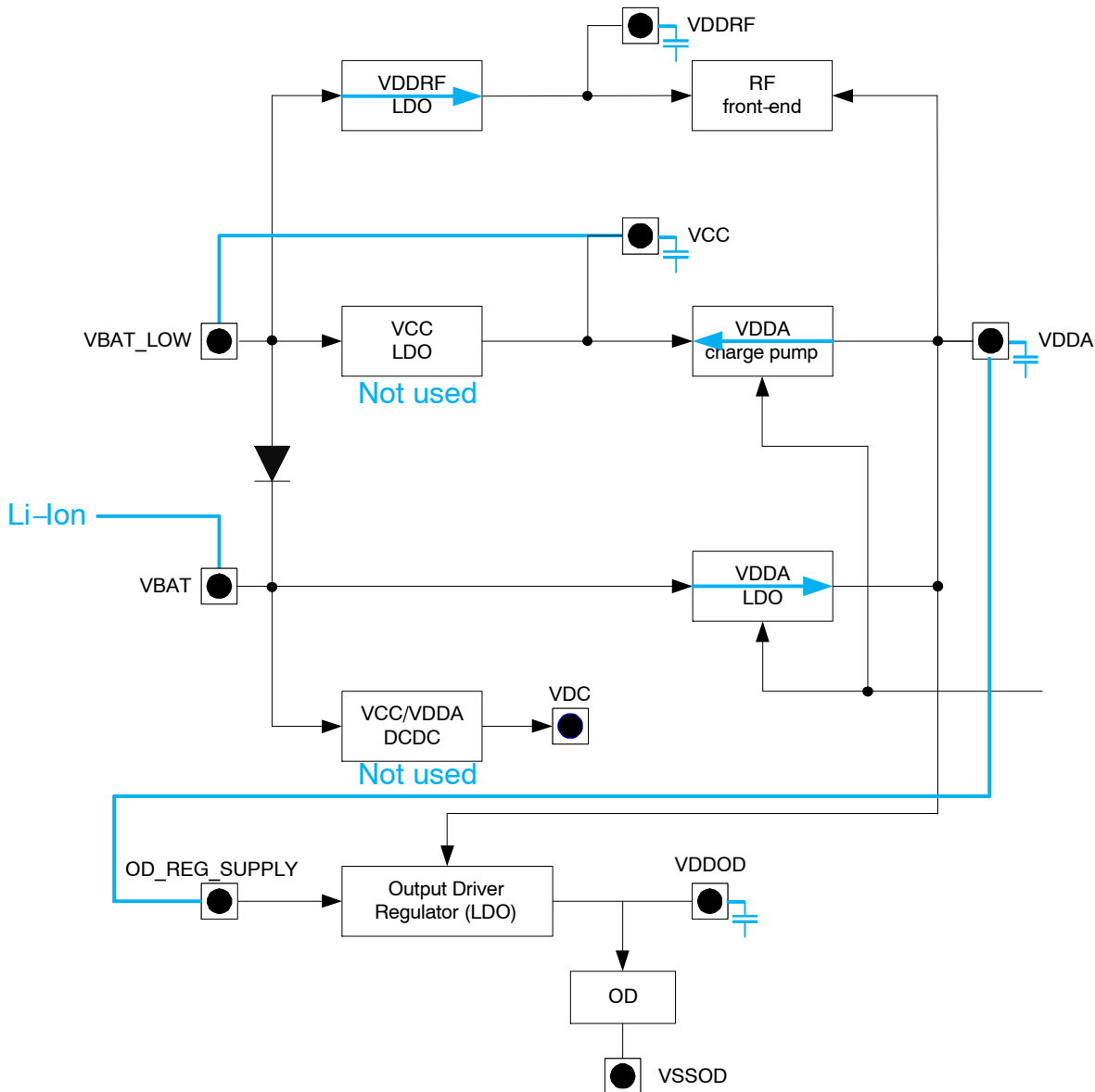
Figure 7. Li-Ion LDO Supply Configuration Diagram
