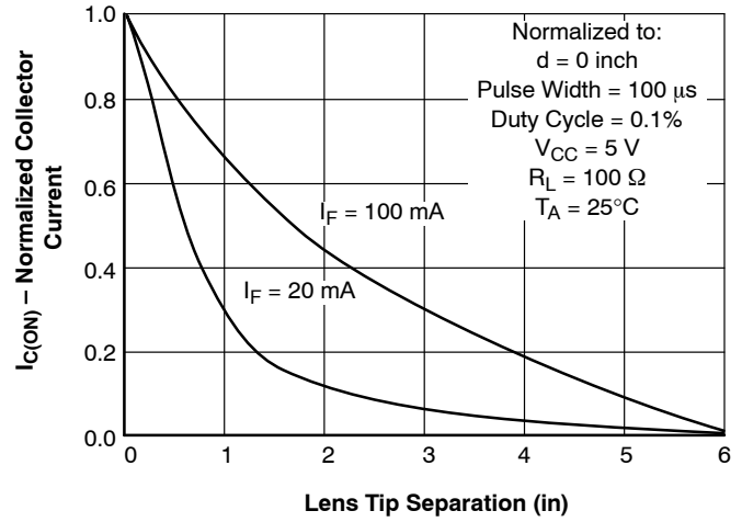
Figure 8. Coupling Characteristics of QED22X and QSD22X
