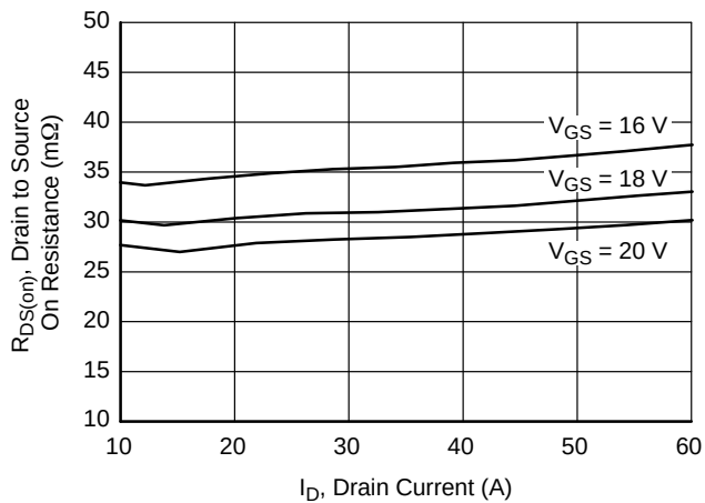
Figure 7. On-Resistance vs. Drain Current
