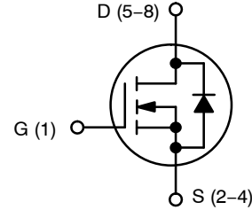
N-CHANNEL MOSFET
