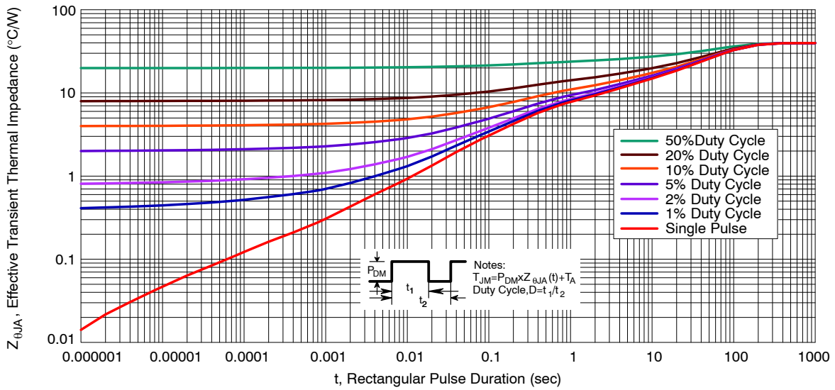
Figure 13. Thermal Characteristics
