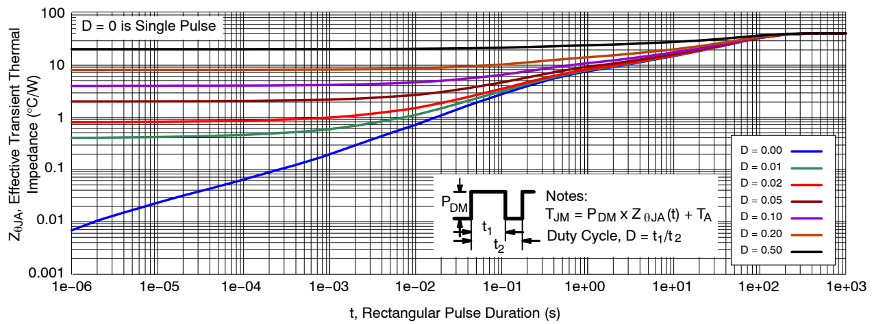
Figure 14. Thermal Response
