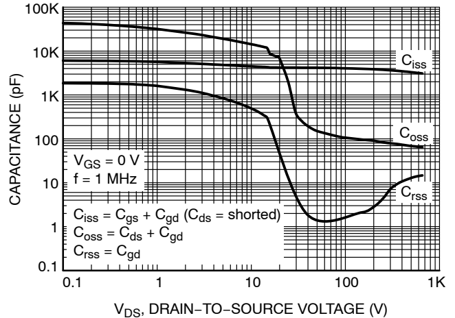
Figure 6. Capacitance Characteristics
