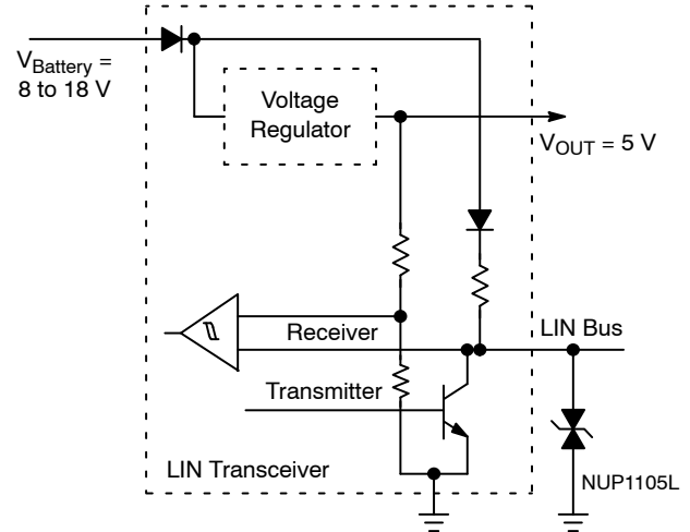
Figure 6. LIN Transceiver
