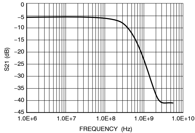
Figure 4. Insertion Loss Characteristic
