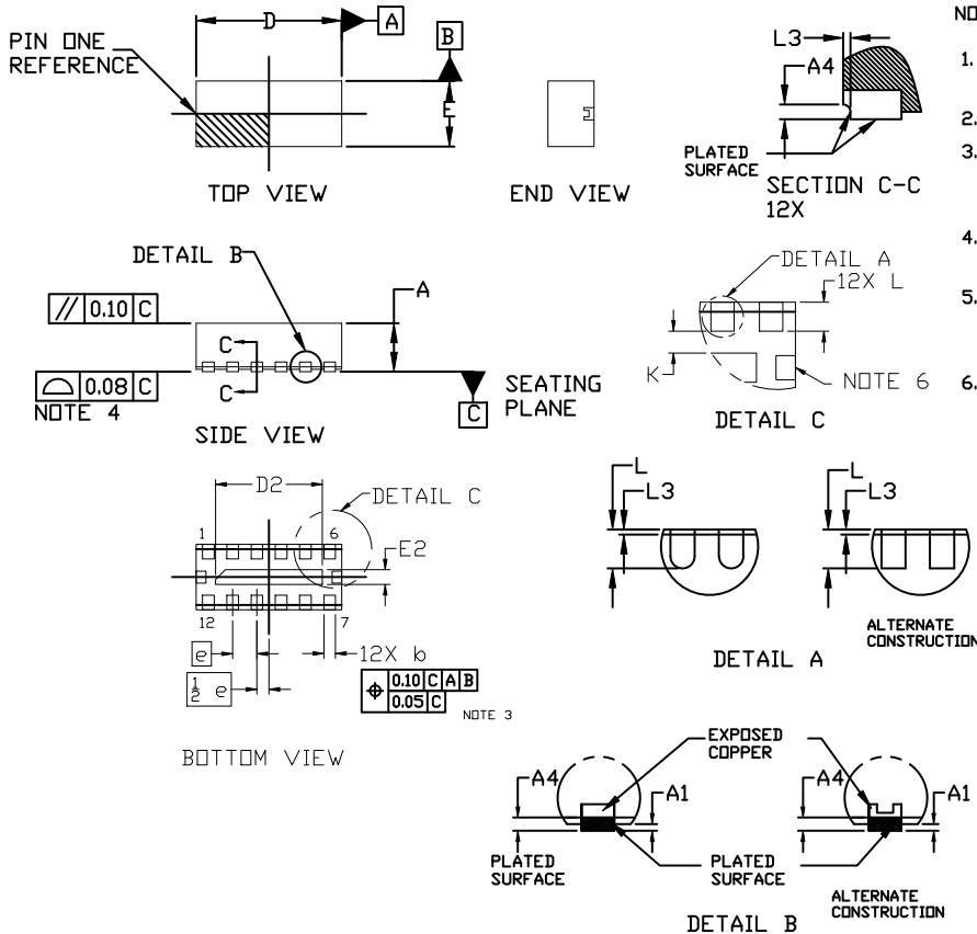
DFNW12 3x1.35, 0.5P CASE 507AY ISSUE 0
