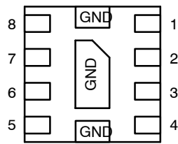
Figure 3. Pin Diagram
