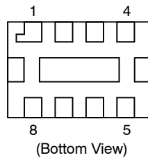
Figure 3. Pin Diagram
