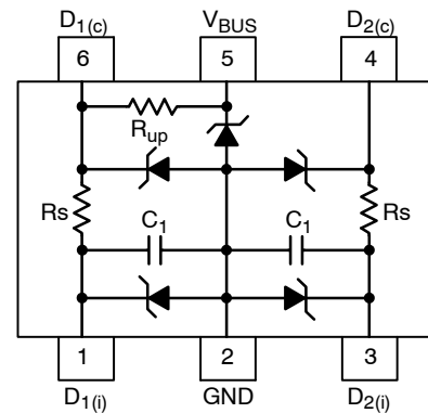
SC-88 / SOT-363 CASE 419B PLASTIC
