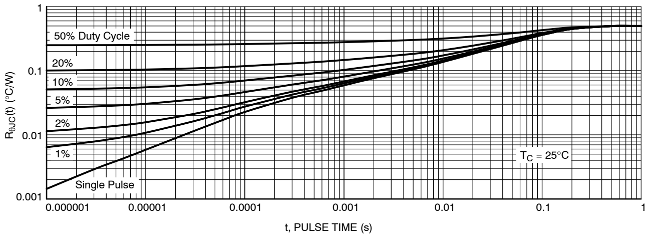
Figure 14. Thermal Response
