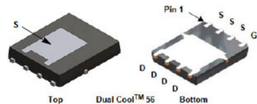
DFN8 5x6.15 CASE 506EG
