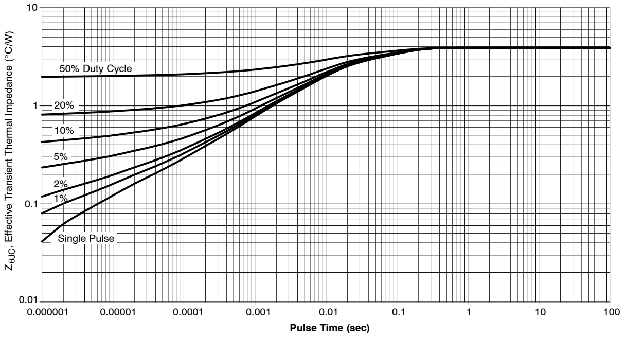
Figure 13. Transient Thermal Response
