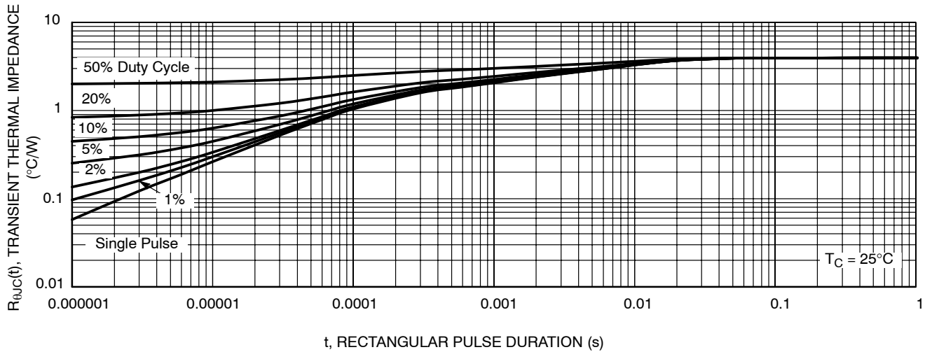
Figure 14. Thermal Response
