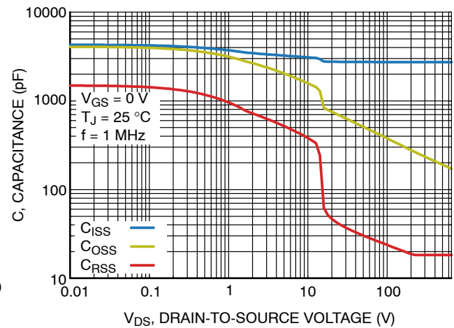
Figure 10. Capacitance Characteristics
