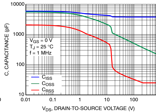
Figure 10. Capacitance Characteristics
