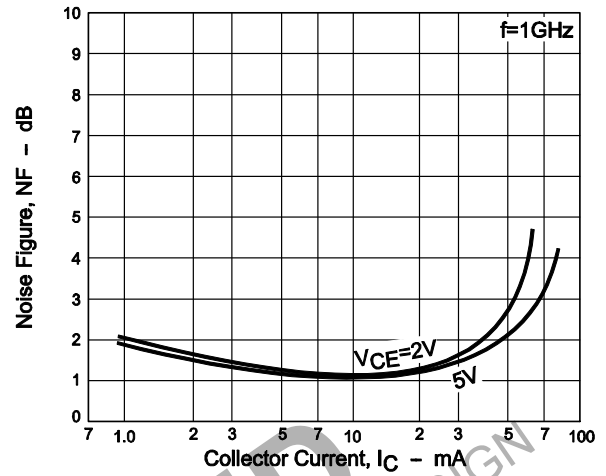
Figure 8. NF - I_C
