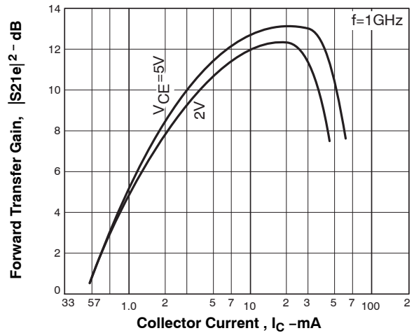
Figure 6. |S_{21e}|^2 - I_C
