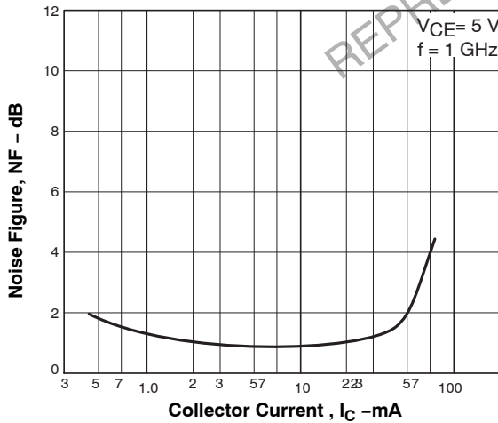
Figure 5. NF - I_C
