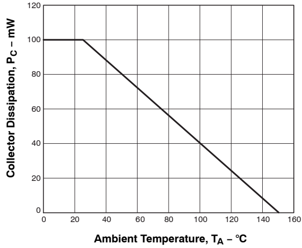
Figure 7. P_C - T_A
