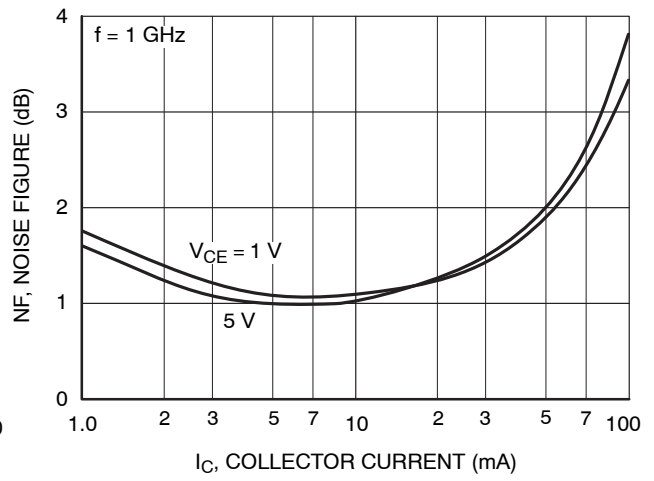
Figure 8. NF - I_C
