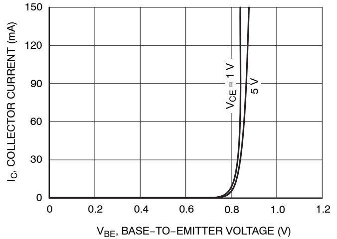
Figure 2. I_C - V_{BE}
