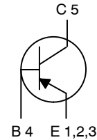
Schematic
