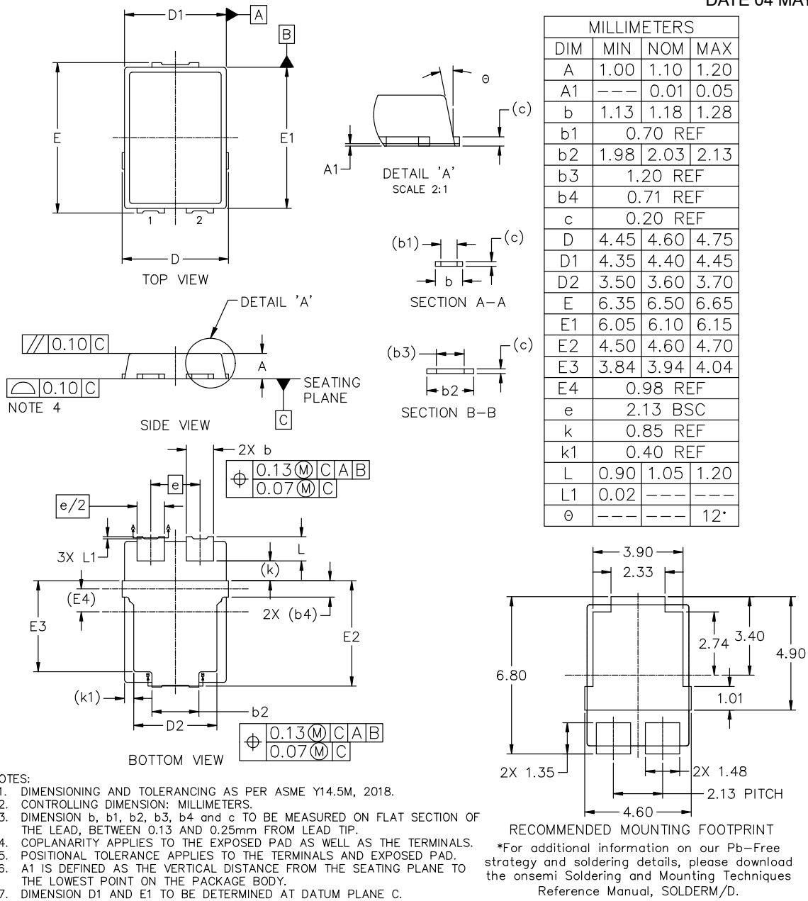
TO-277-3 4.40x6.10x1.10, 2.13P CASE 340CZ ISSUE B
