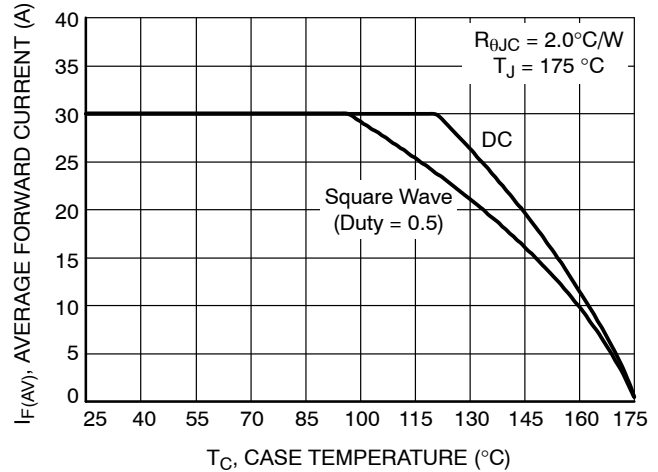
Figure 4. Current Derating
