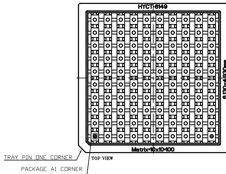
Figure 45. Pin 1 Location
