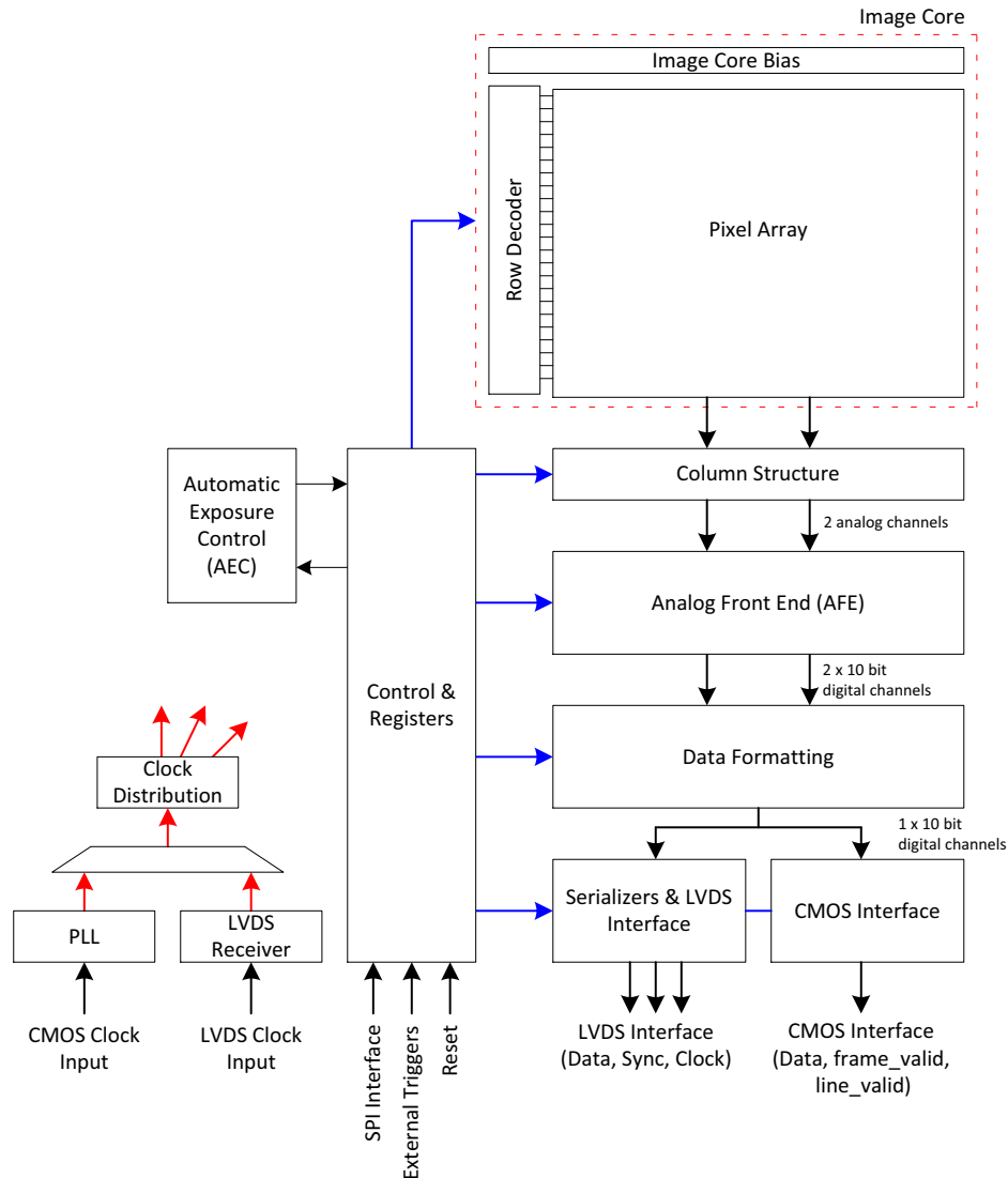
Figure 11. Block Diagram
