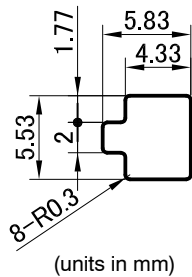
Figure 47. Dimensions of the Protective Foil
