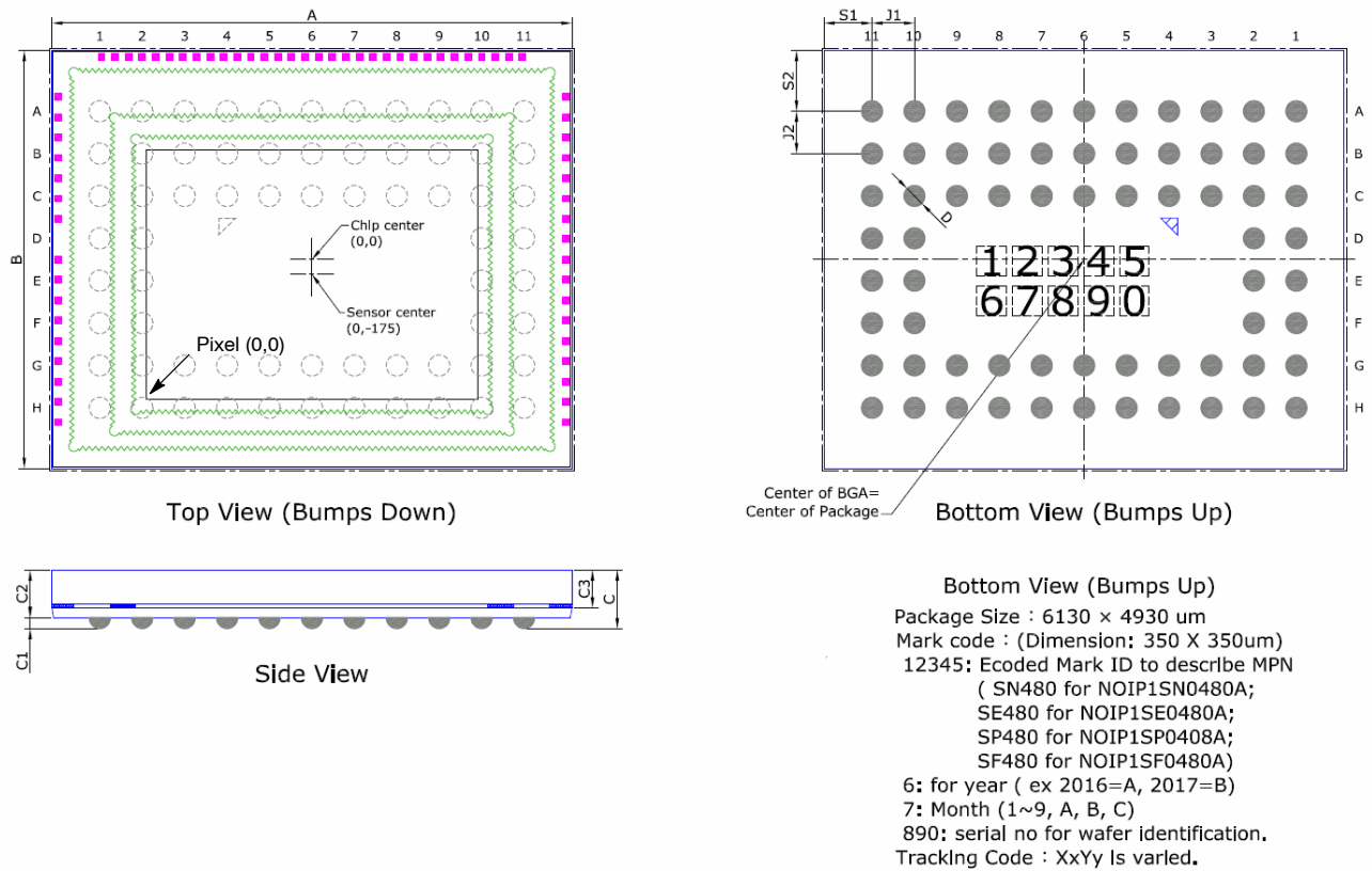
Figure 43. Mechanical Diagram
