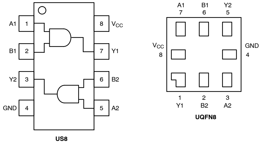
Figure 2. Pinout
