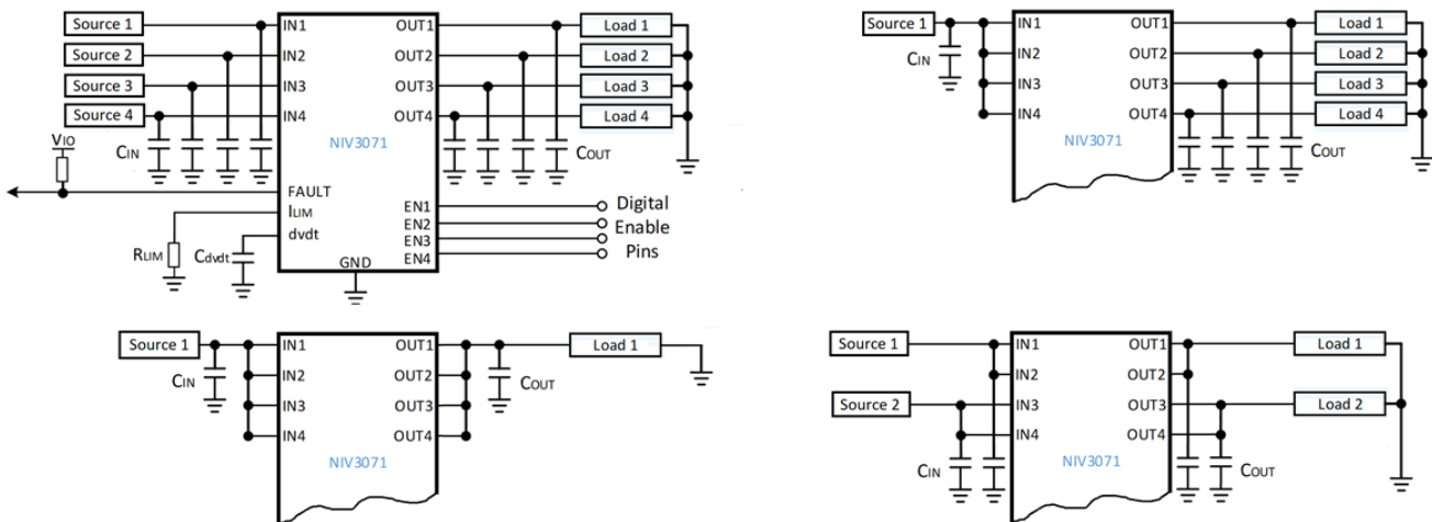
Figure 2. Application Diagrams
