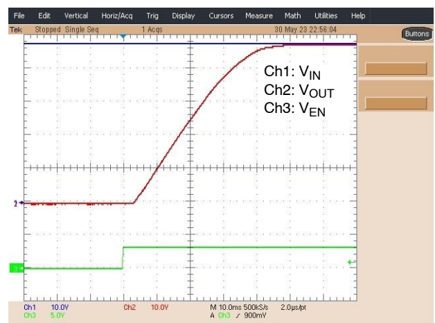
Figure 17. Turn On with EN Pin with C_{dvd1} 56 pF
