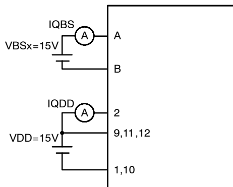
Figure 20. Test Circuit for I D
