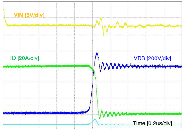
Figure 26. Turn-off Switching Waveform
